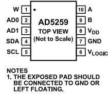
Figure 5. Pin Configuration
