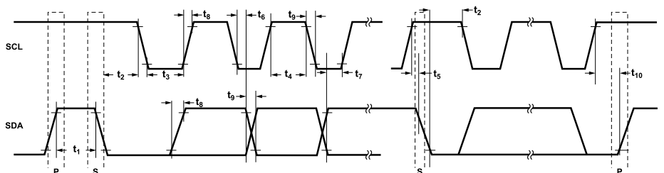
Figure 4. I 2 C Interface Timing Diagram
