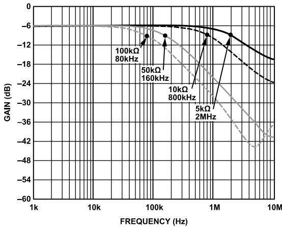
Figure 26. -3\text{ dB Bandwidth @ Code} = 0x80
